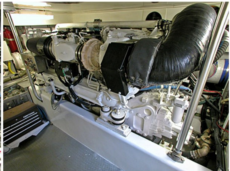
engineroom2_starboard_engine.jpg
