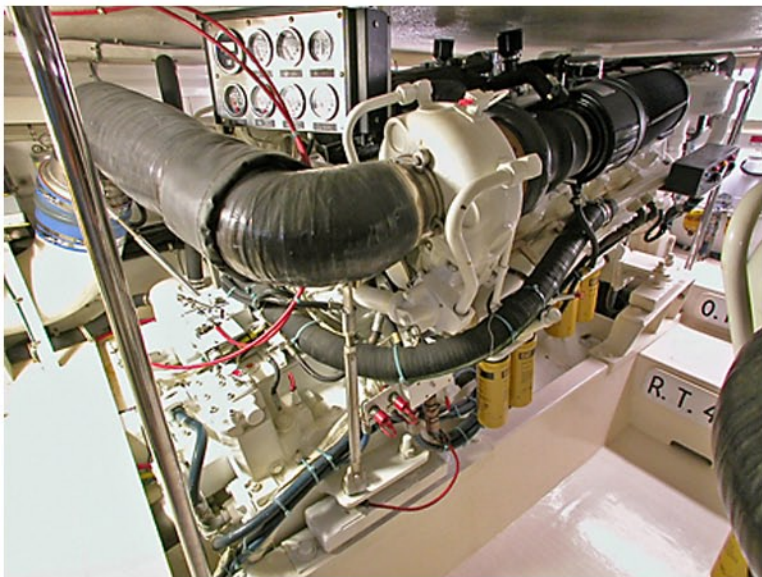
engineroom3_port_engine.jpg
