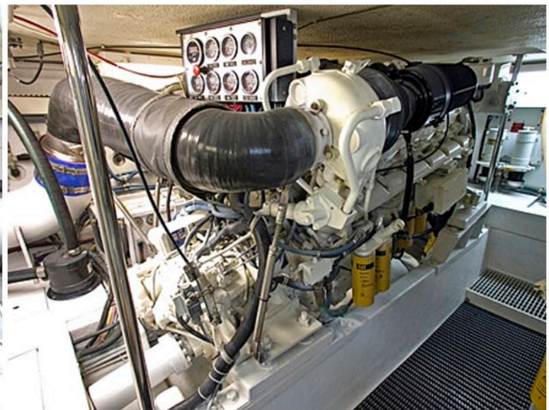
engineroom3_port_engine.jpg
